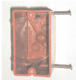
1099-NRED Single gang 22.5 cu. in. 3 9/16" x 2 1/4" x 3 3/4" Angled mid-nails
