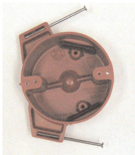
9351-NKRED 4/0 round ceiling 22.5 cu. in. 2 3/8" x 4" dia. Fetter ring nails, Speed Klamps™
