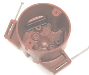
9335-NKRED 3/0 round ceiling 20.5 cu. in. 3 7/8" x 3 1/2" dia. Fetter ring nails, Speed Klamps™
