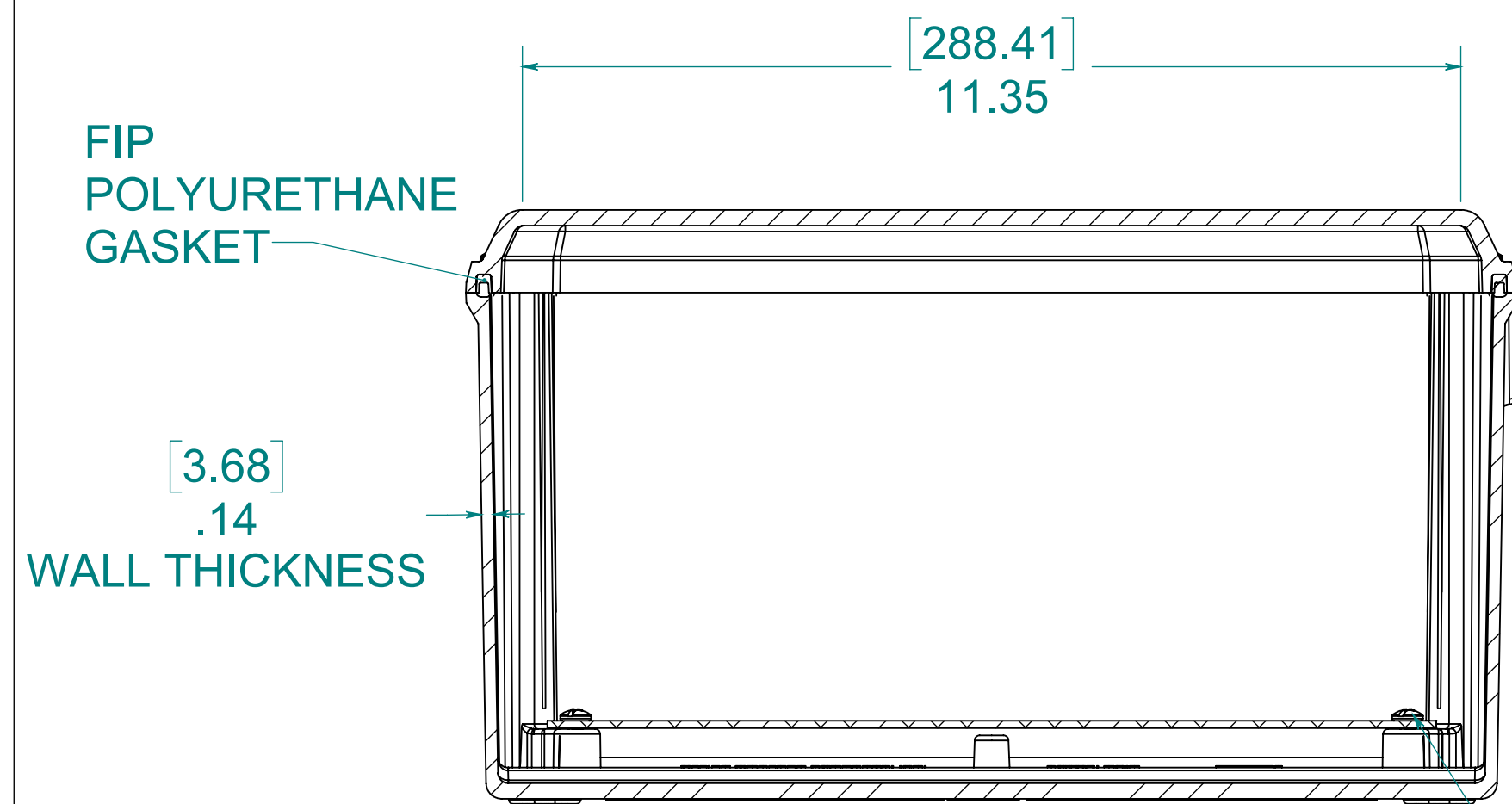
SECTION B-B
